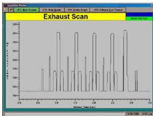
InspeXion Screen showing a Profile Scan Waveform of the Entire Cylinder Head
